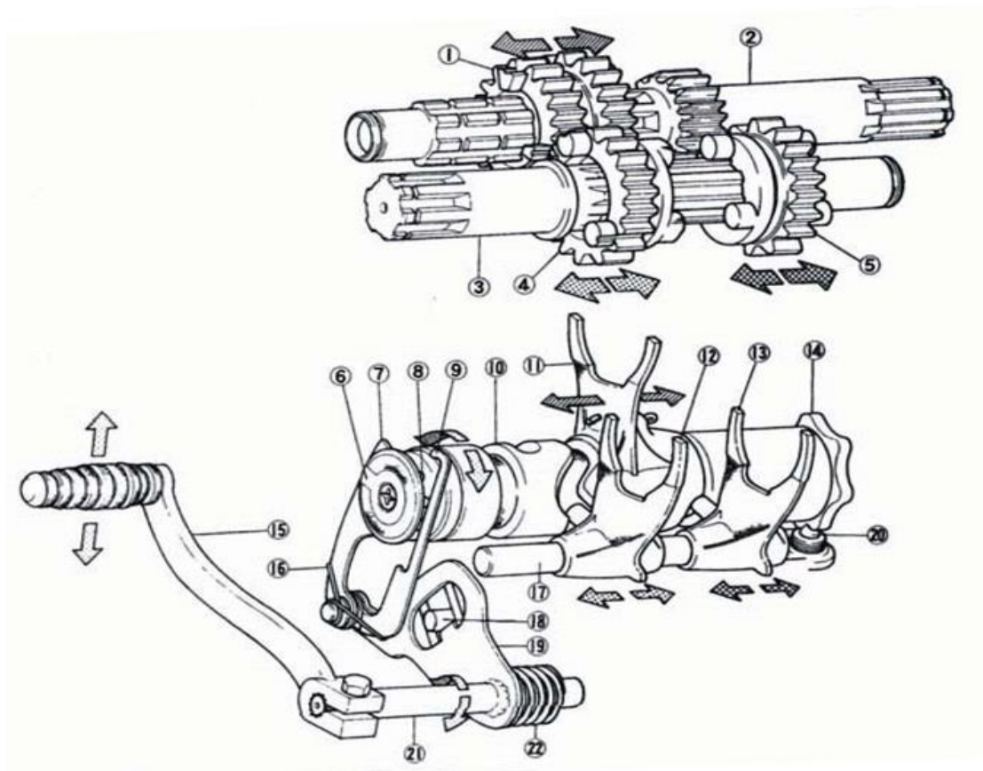
Gambar 2.8 Transmisi Manual (Jama, 2008)
