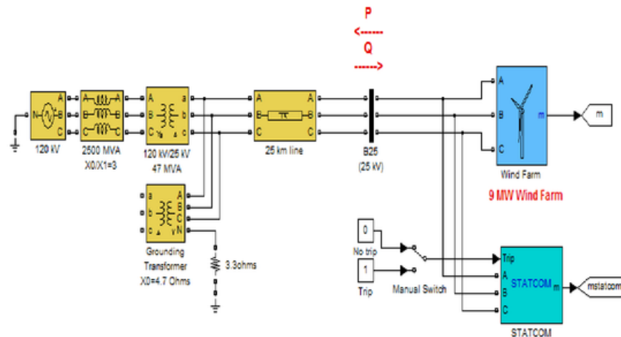
Fig. 3. Wind turbines connected to a distribution system.
