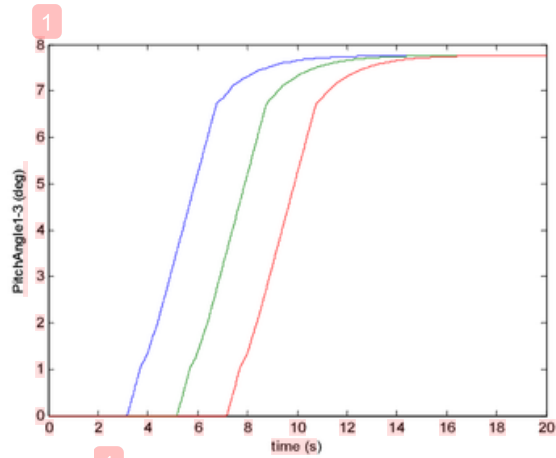
Fig 7. Change of wind turbine pitch angle.
