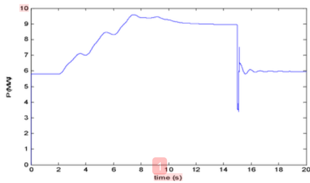
Fig. 18. Active power of bus B25 under fault condition
