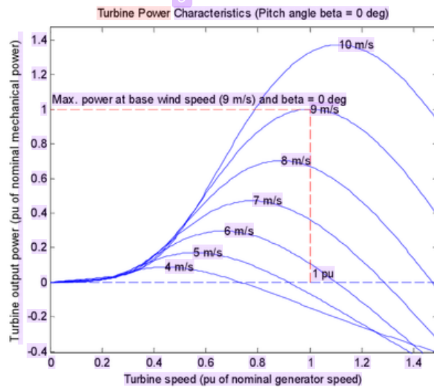
Fig. 6. Wind turbine characteristics with pitch angle of 0^\circ .
