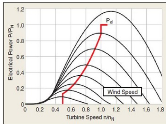
Fig.1. A common characteristic of wind turbines [13]
