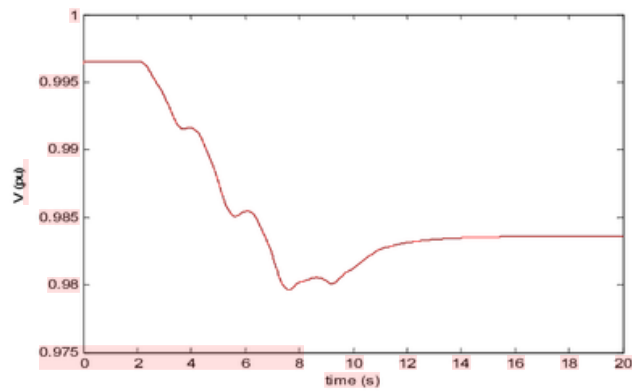
Fig.10. Voltage of bus B25 under normal condition.
