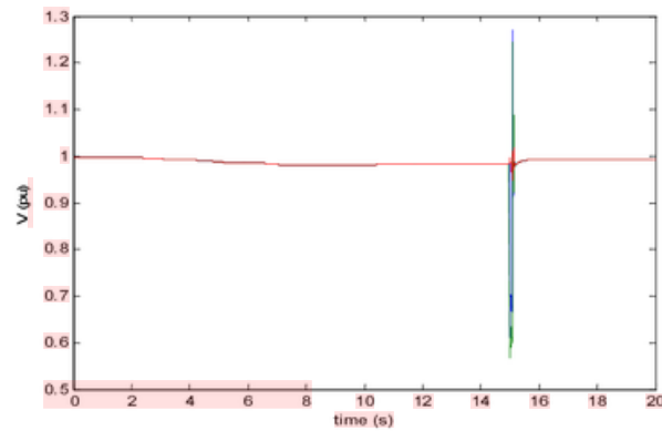
Fig. 17. Bus voltage under fault condition
