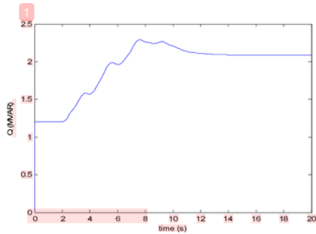
Fig.12. Reactive power of bus B25 under normal condition
