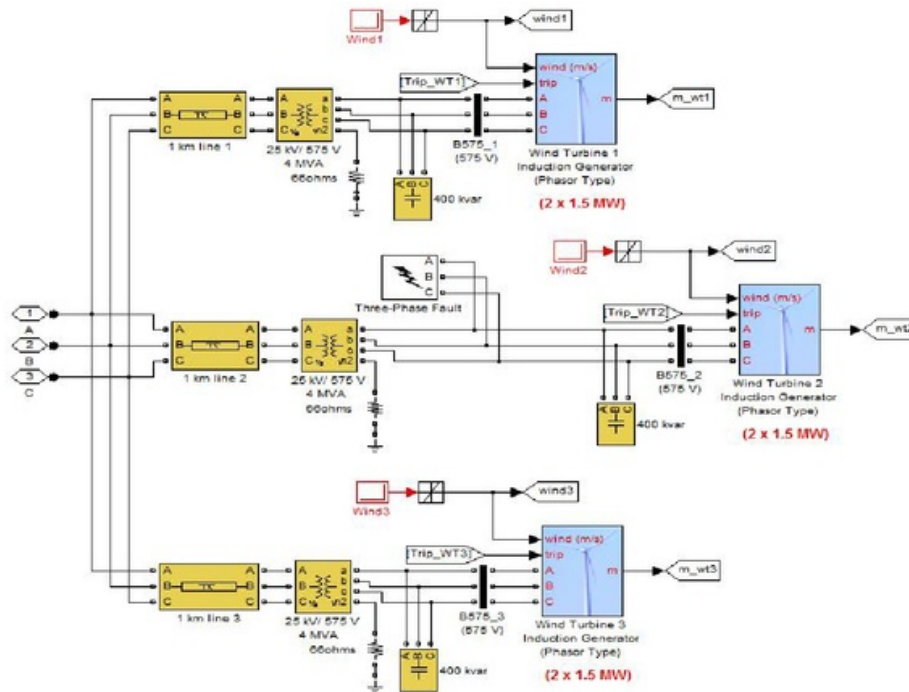
1 Fig 4. Wind turbines model.
