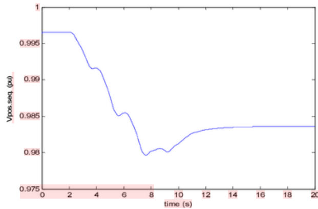
Fig.13. Positive sequence voltage of bus B25 under normal condition
